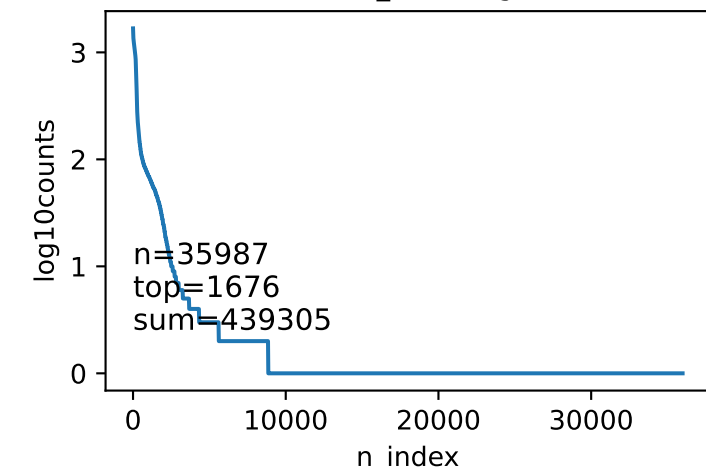
BC22 read_count log10().
